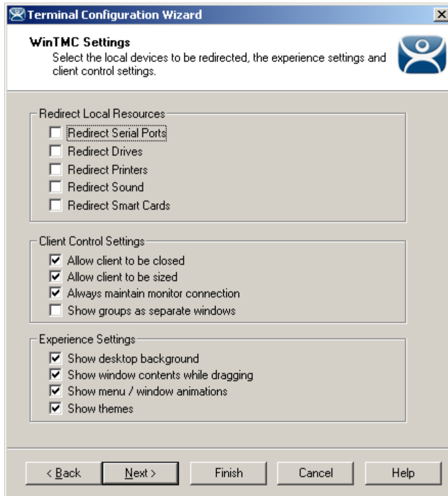
WinTMC Settings
