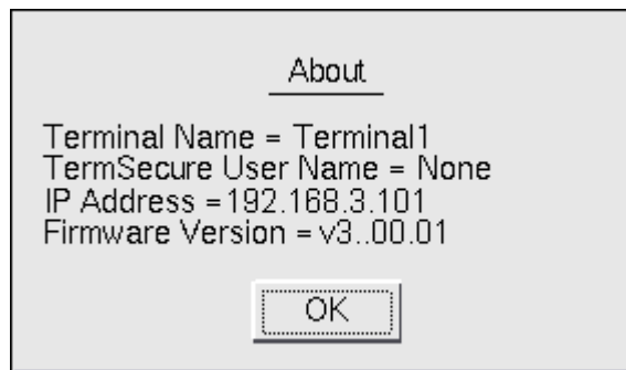
About Menu
