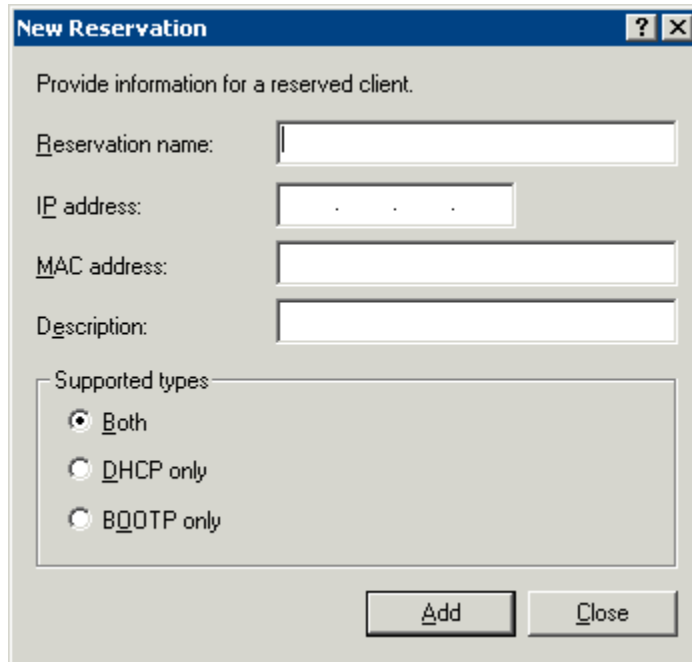
Scope Reservation
