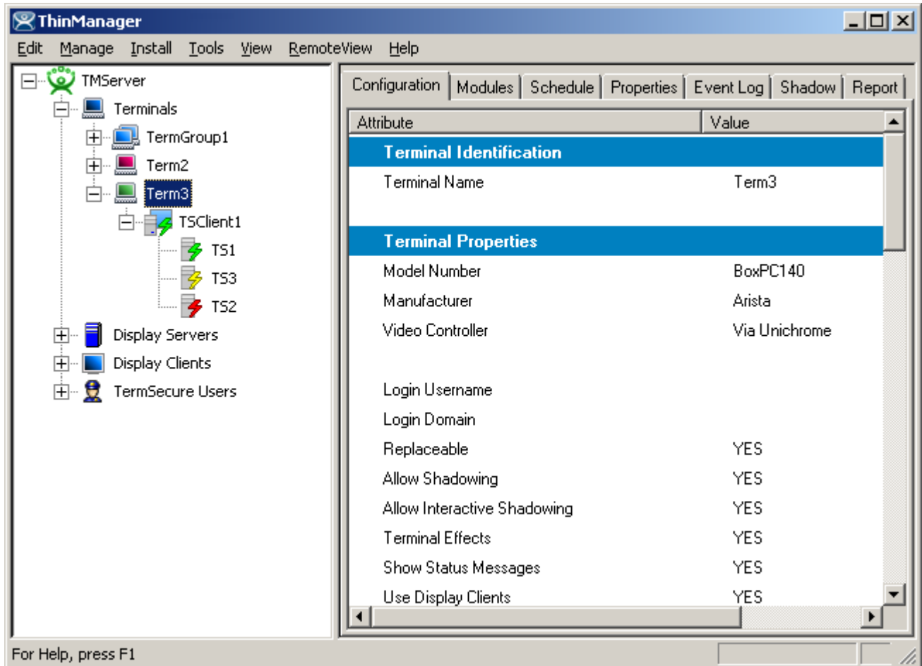
Instant Failover
