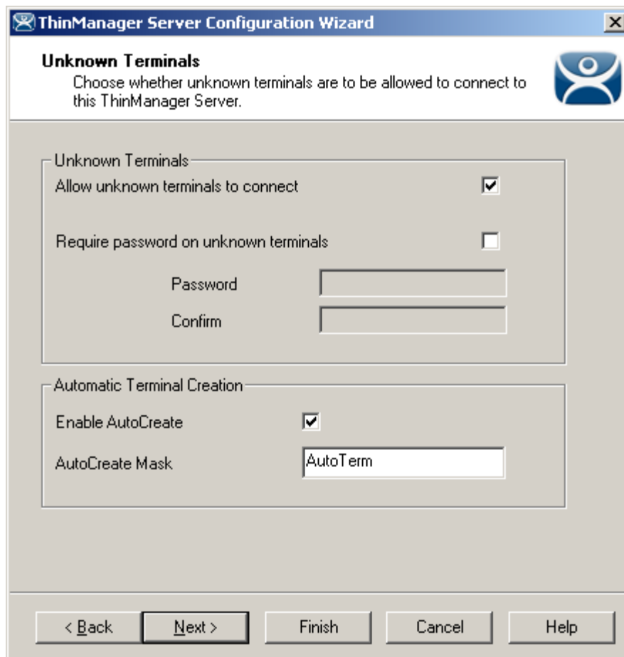
Unknown Terminals
