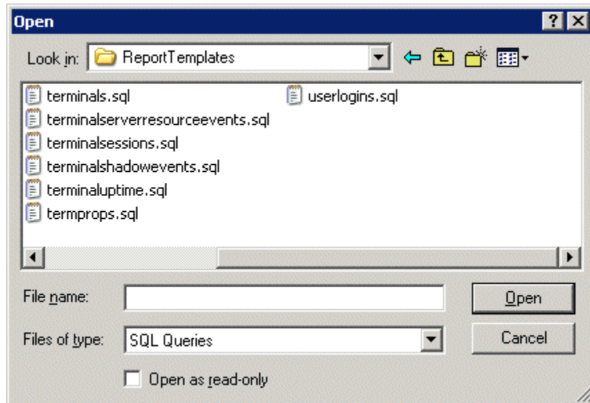
File Browser
