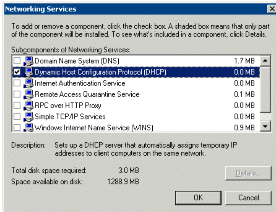
Networking Services
