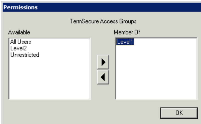
Object Permissions
