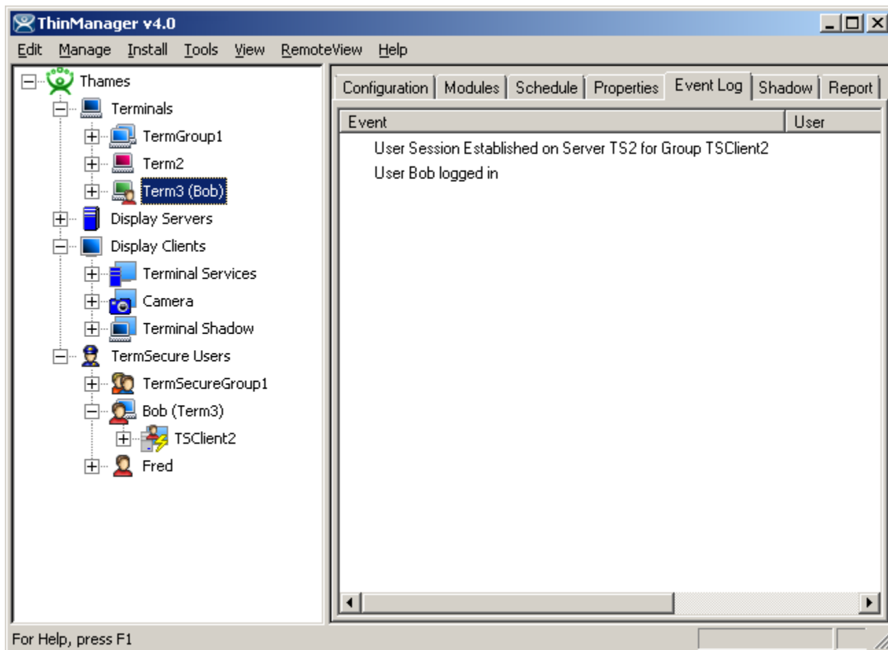
Event Log
